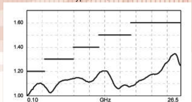
Typical V.S.W.R.
